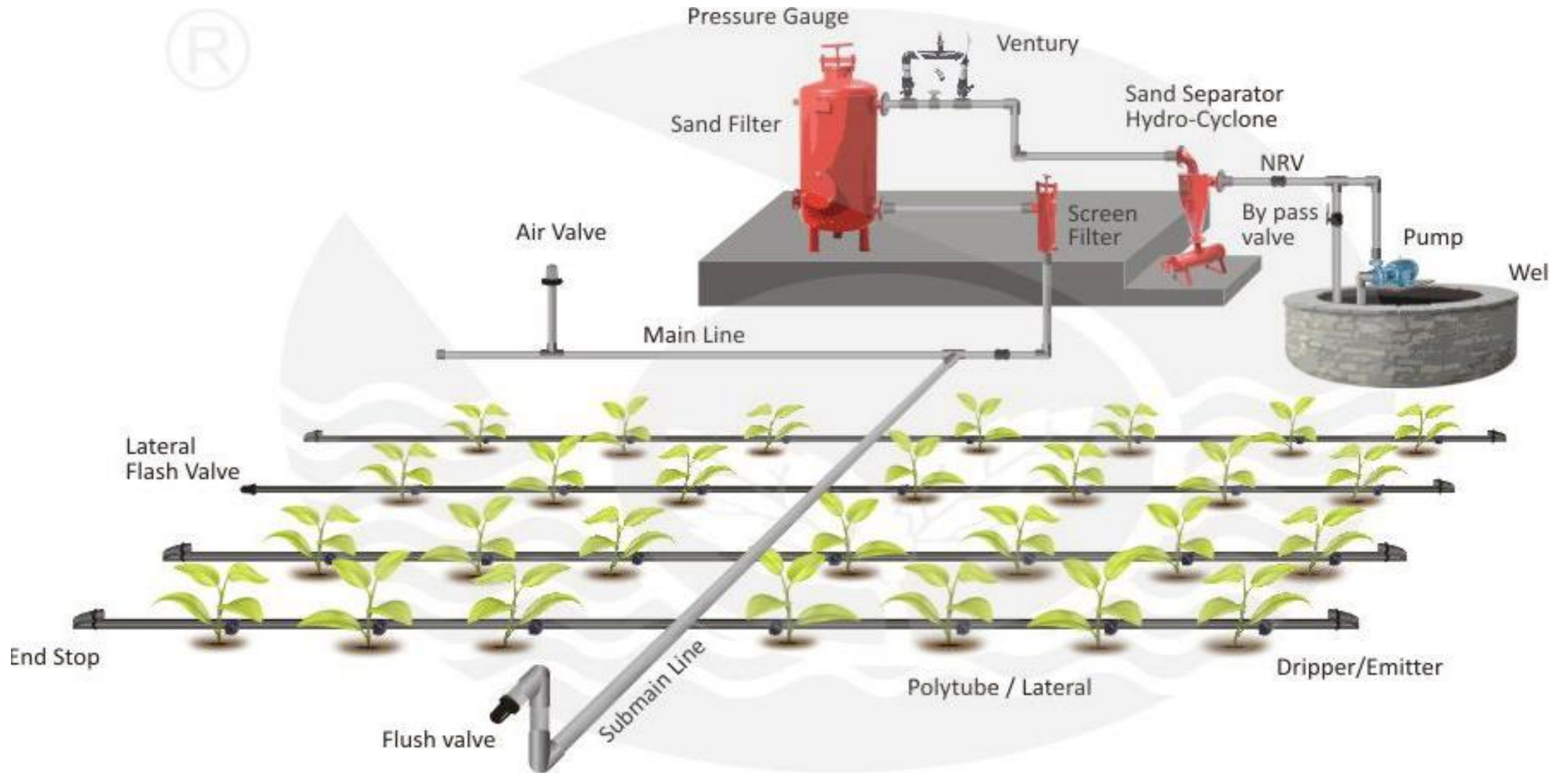
Drip Irrigation System
